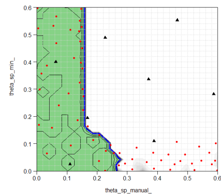
For two control parameters, estimation (in green) of the NH 3 emission standard compliance set (initial simulated points in black, points added via the iterative method in red).
